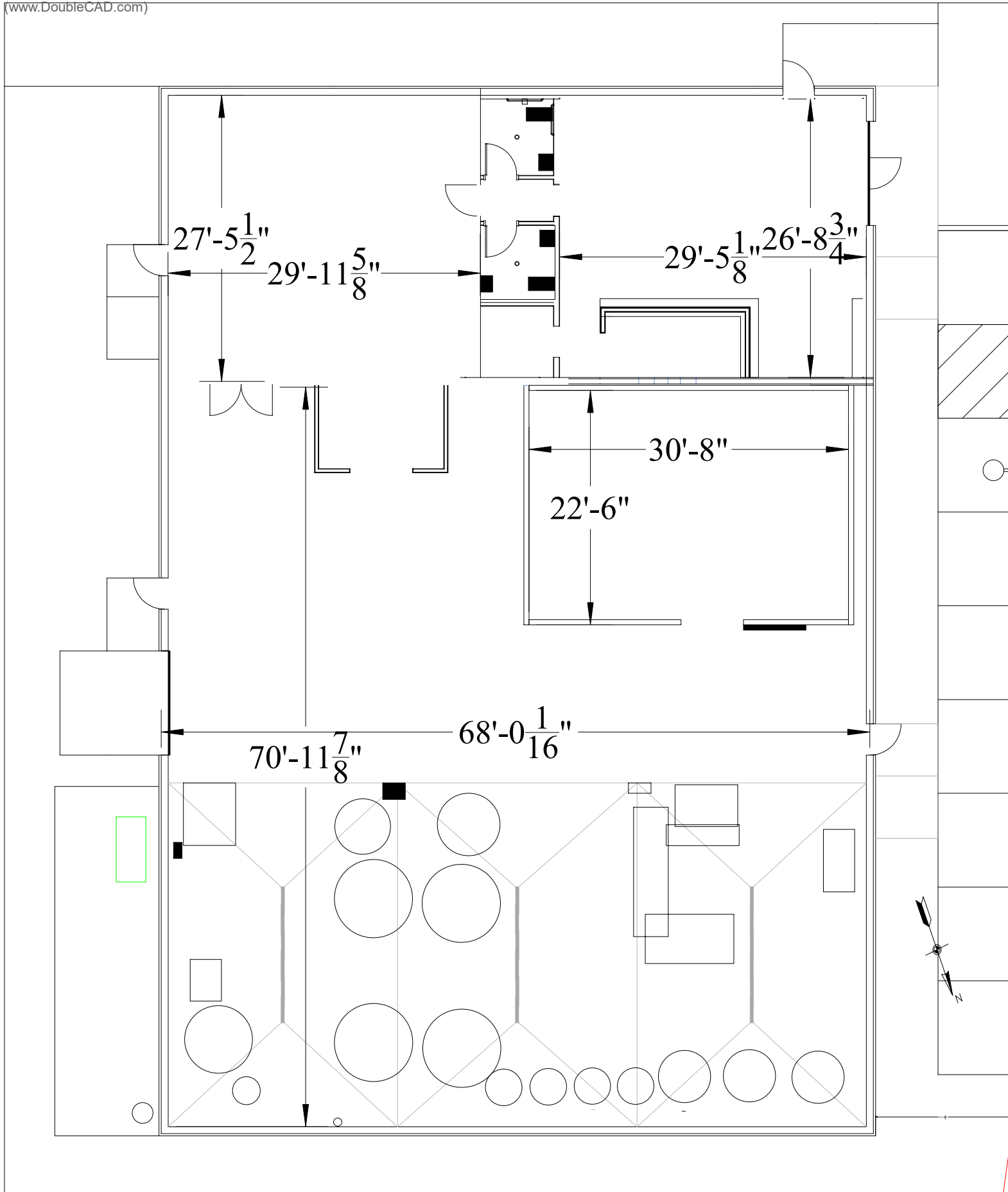
Existing Structure
